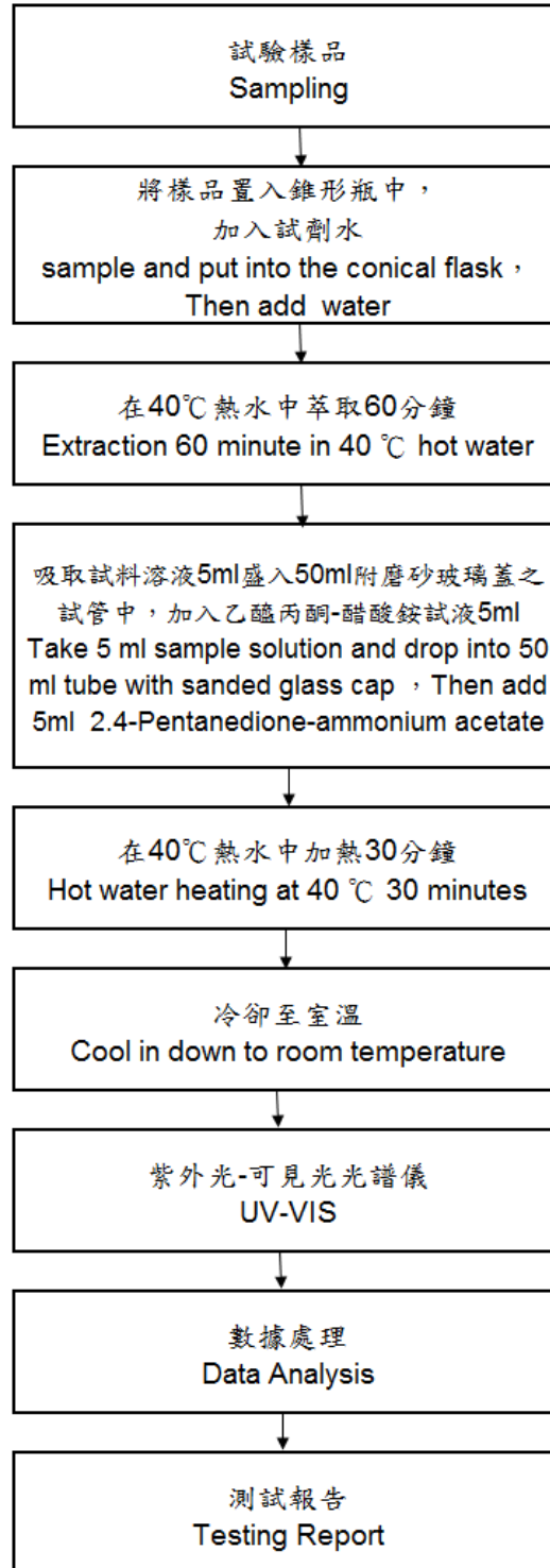
Flow Chart for Formaldehyde
