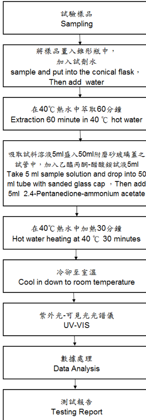
Flow Chart for Formaldehyde
